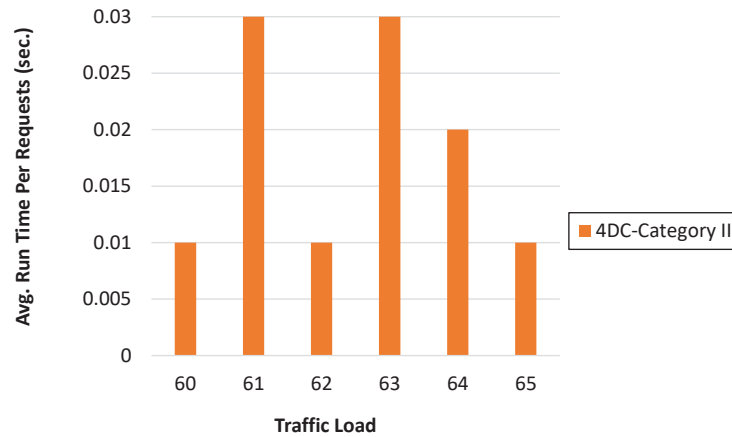
Figure 4.5: Running time per request with different traffic loads for ARPANET with 4 DCs and category II disasters.
