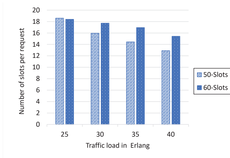
Figure 5.7: Resource utilization obtained by proposed approach for 14-node NSFNET network with 2 DCs and 4 cores per fiber link.
